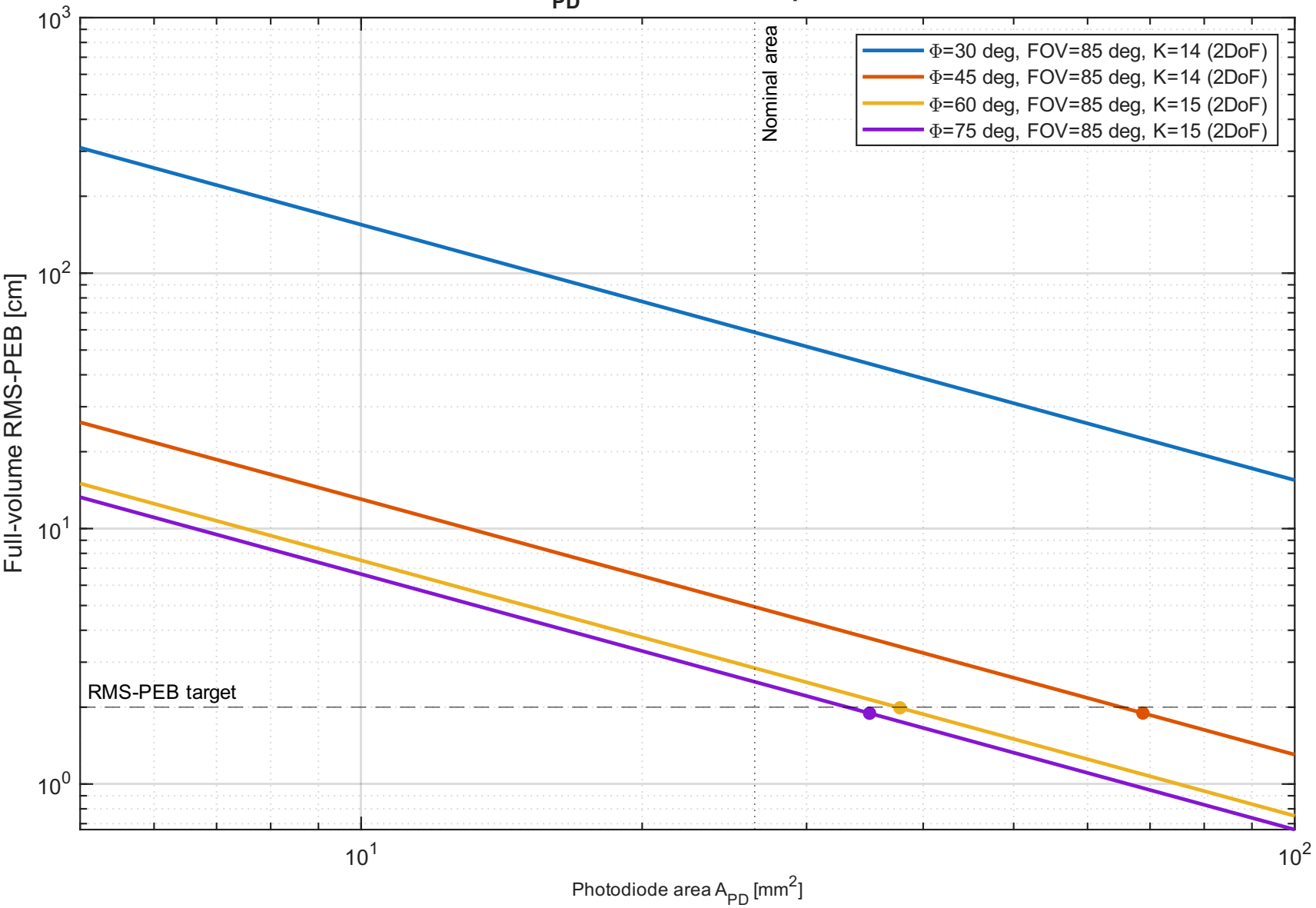
Locally refined 2DoF orientations; constant optical noise PEB scales as 1/A_{\text{PD}} : no interior area optimum in this model
